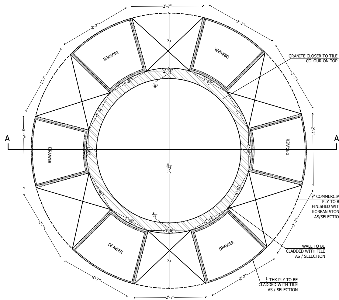
SECTIONAL PLAN
