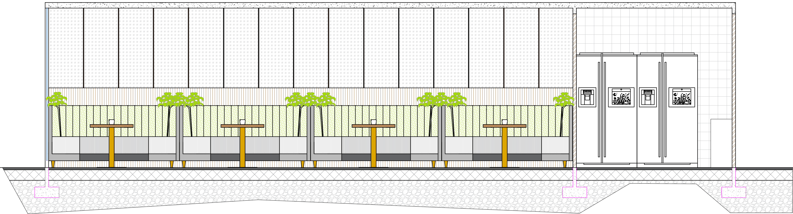
SECTION AA'
